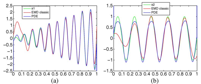
Fig. 3. Comparisons between classical IMFs and \delta -IMFs for the last signal given by (20).
